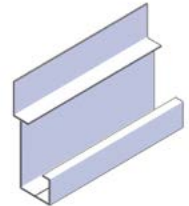
4x8 Gutter w 4 inch Flat Fascia Extension Also available in 4x6, 4x10 and 4x12
