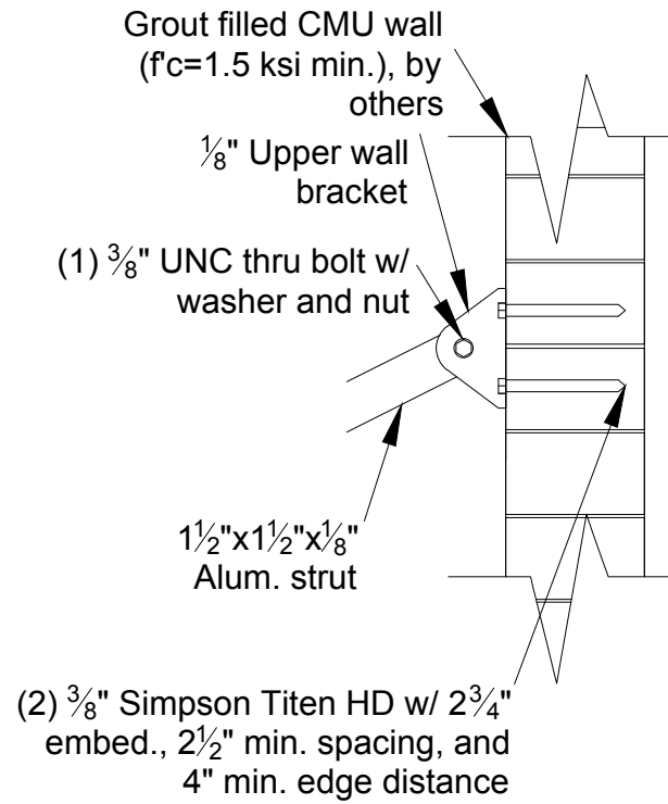
2/10 Wall Bracket Detail
