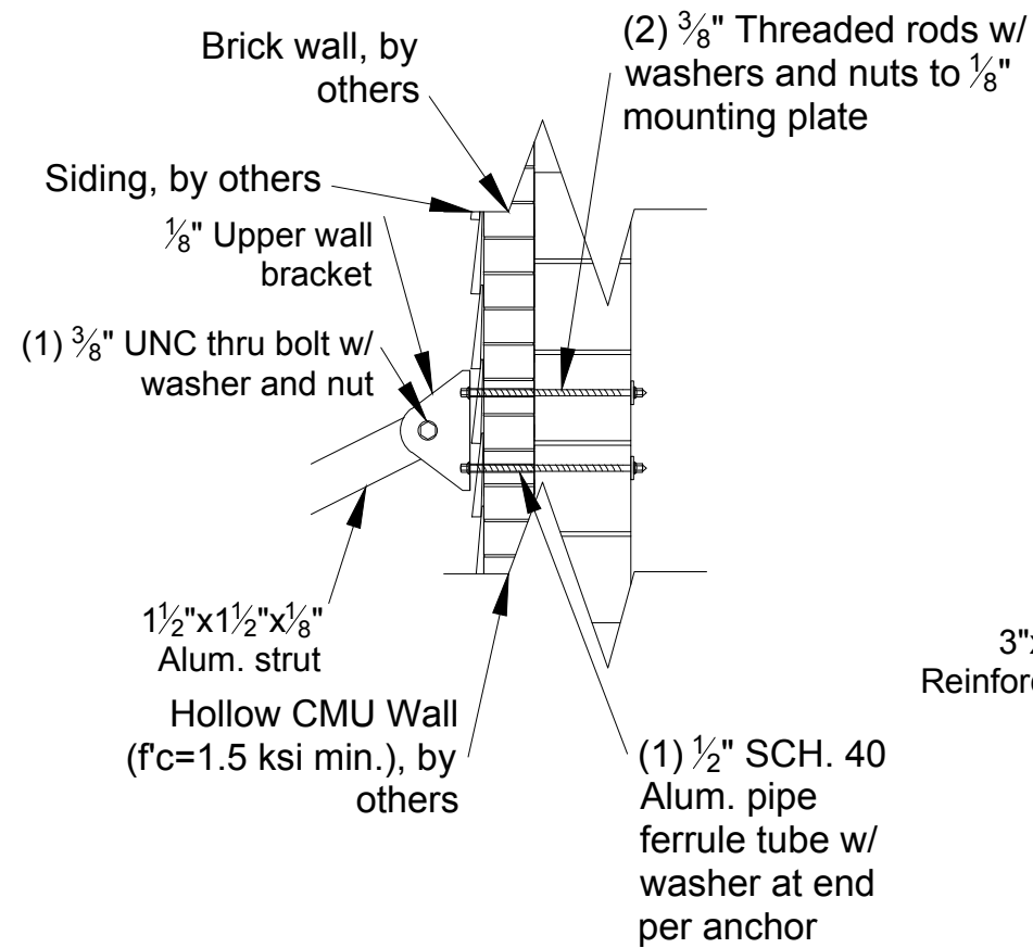
2 12 Wall Bracket Detail
