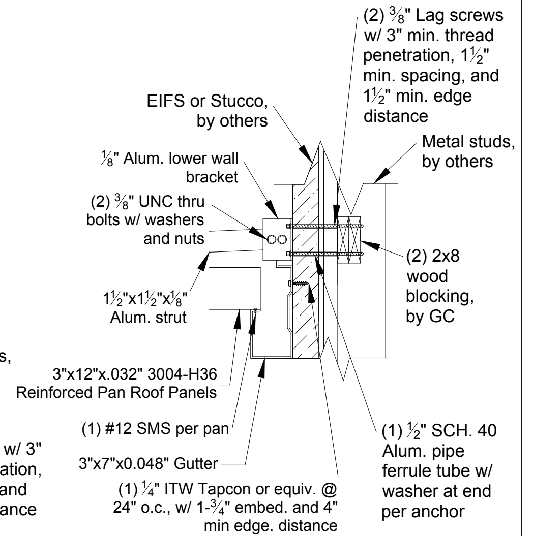
3/13 Rear Gutter Detail
