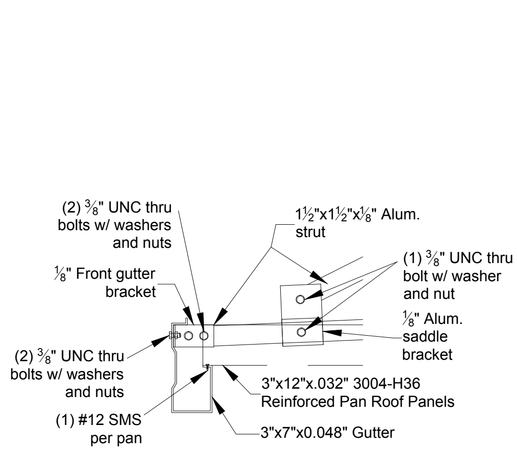
1/13 Front Gutter Detail
