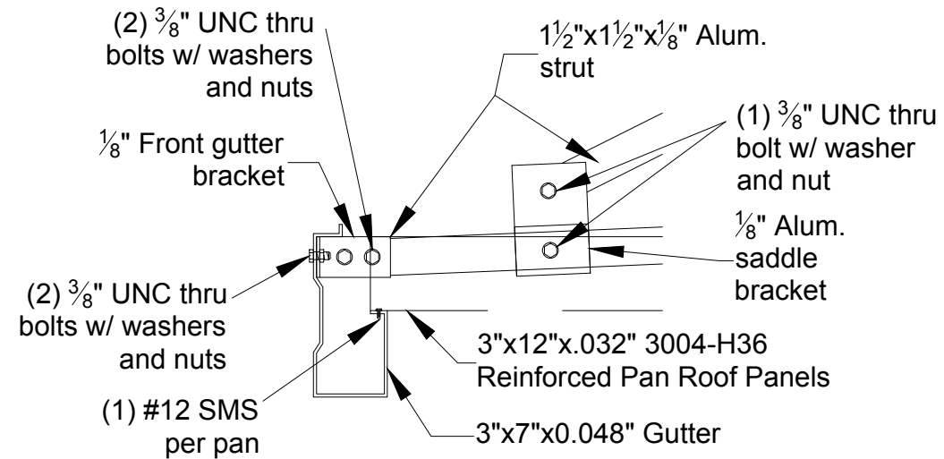
1/9 Front Gutter Detail
