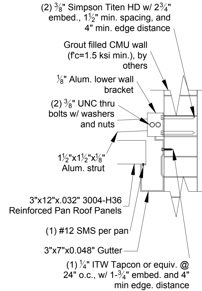
3/10 Rear Gutter Detail
