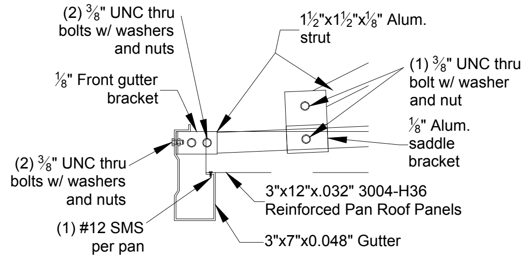
1/11 Front Gutter Detail
