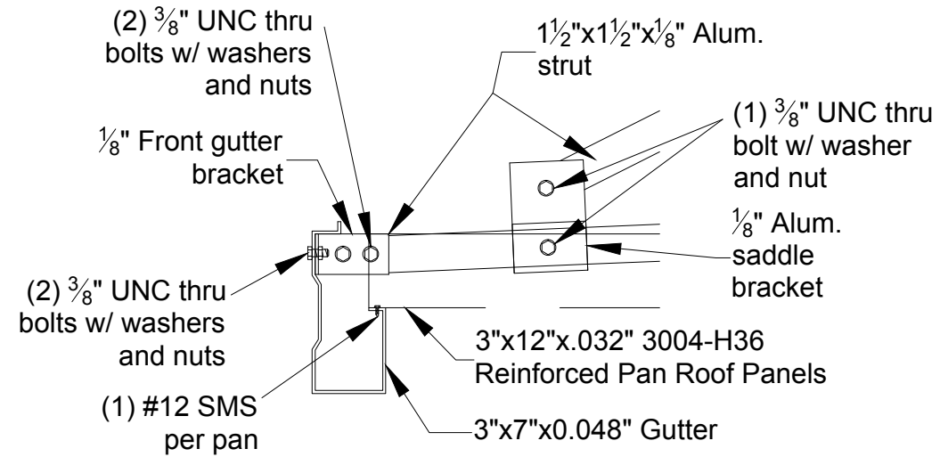
1/10 Front Gutter Detail
