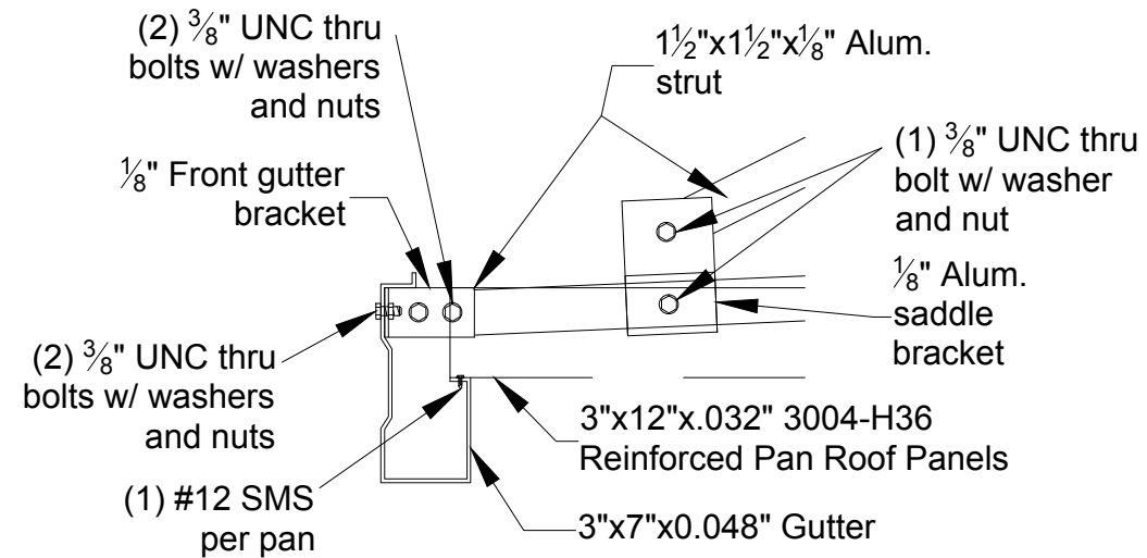
1 12 Front Gutter Detail
